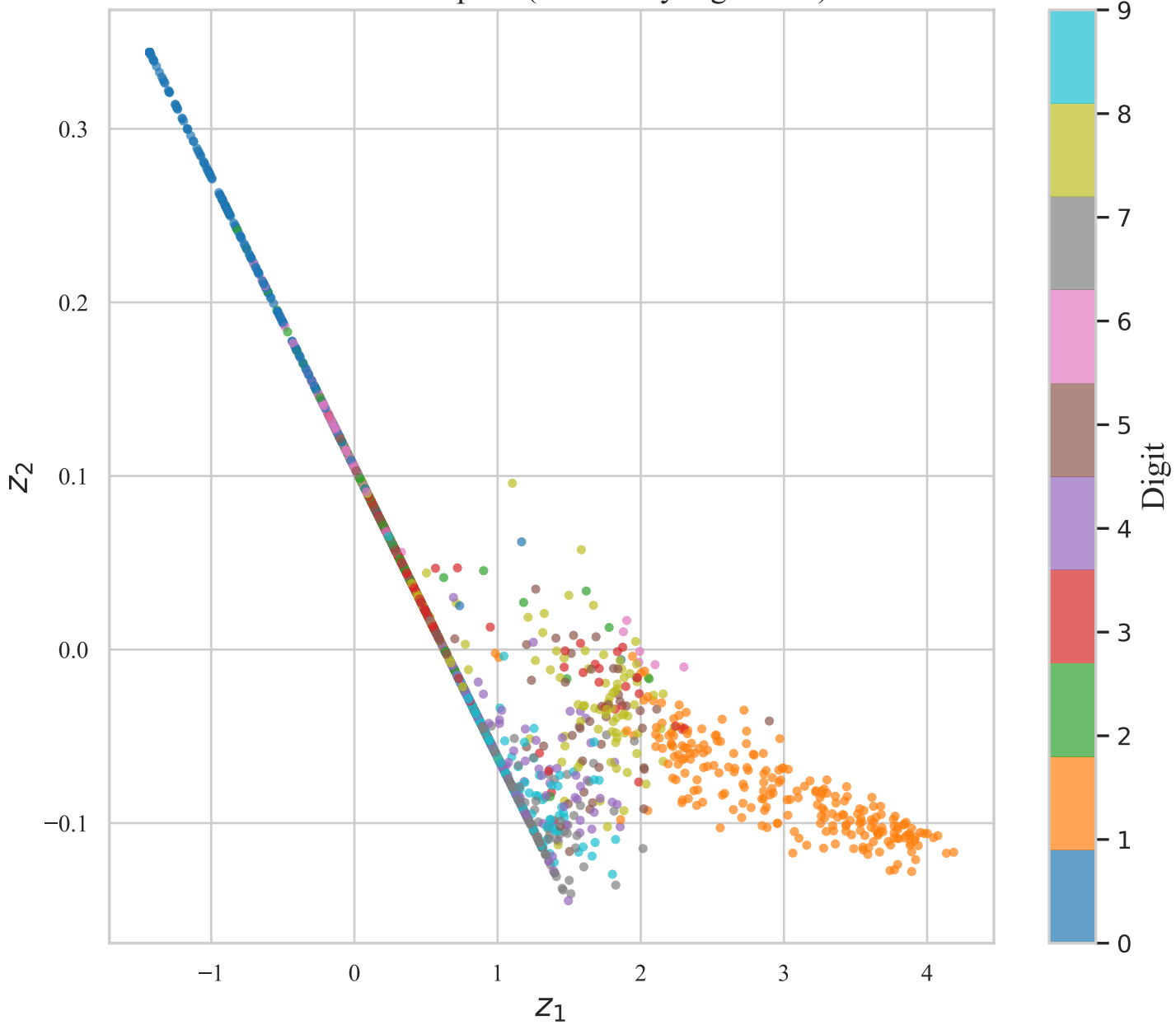
VAE Latent Space (colored by digit label)
